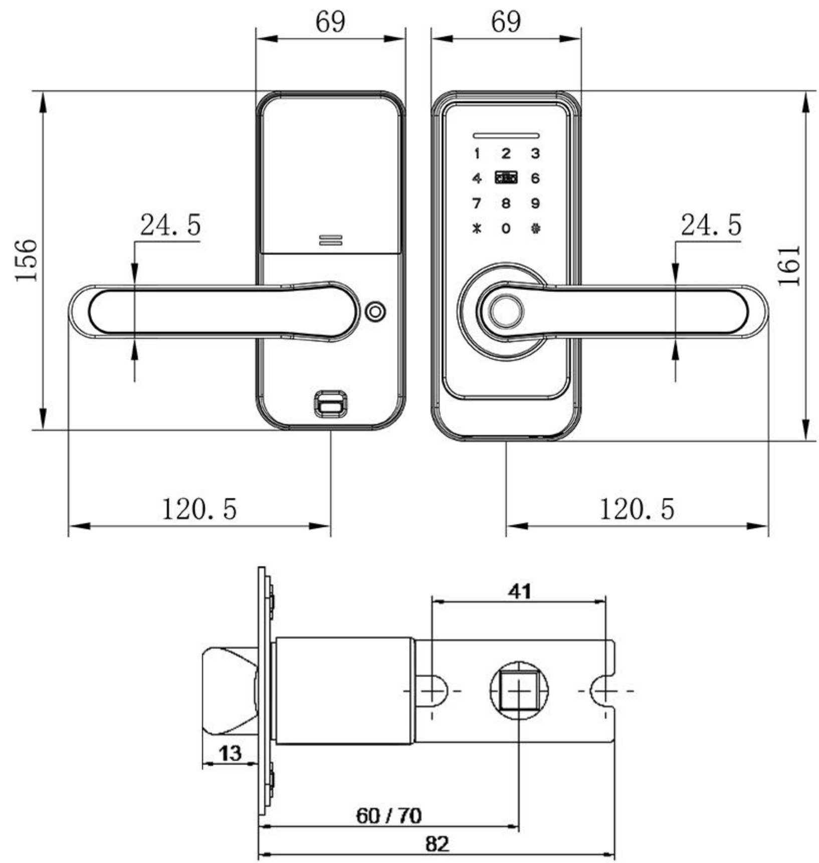
Cylindrical Latch
